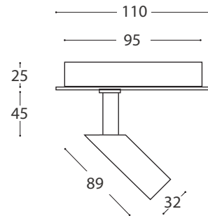
Laser MR8 with built in Transformer 12v 10 - 20w MR8
