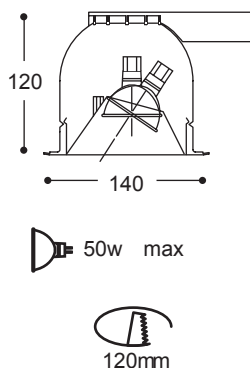
Orli 1 - Pin 12v 20 - 50w MR16
